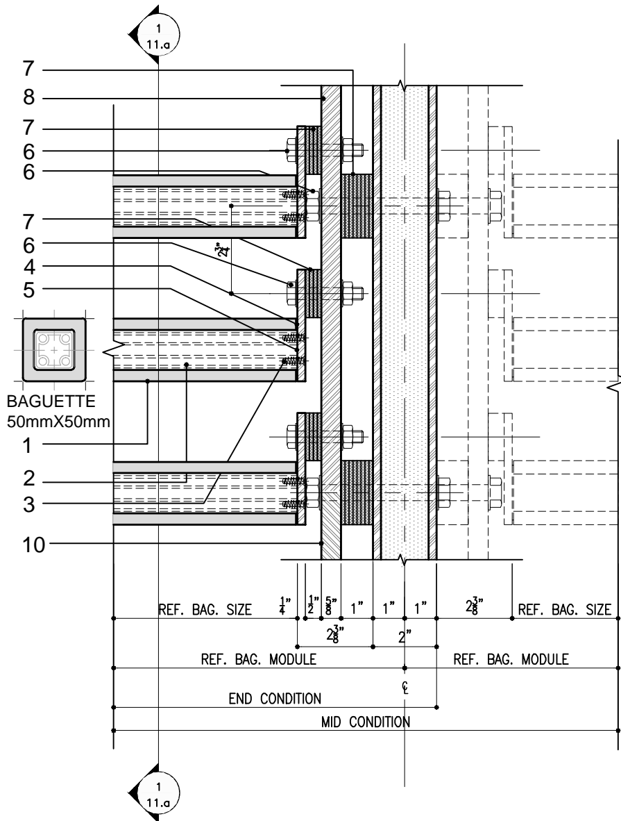
1 PLAN DETAIL-THROUGH TILE
