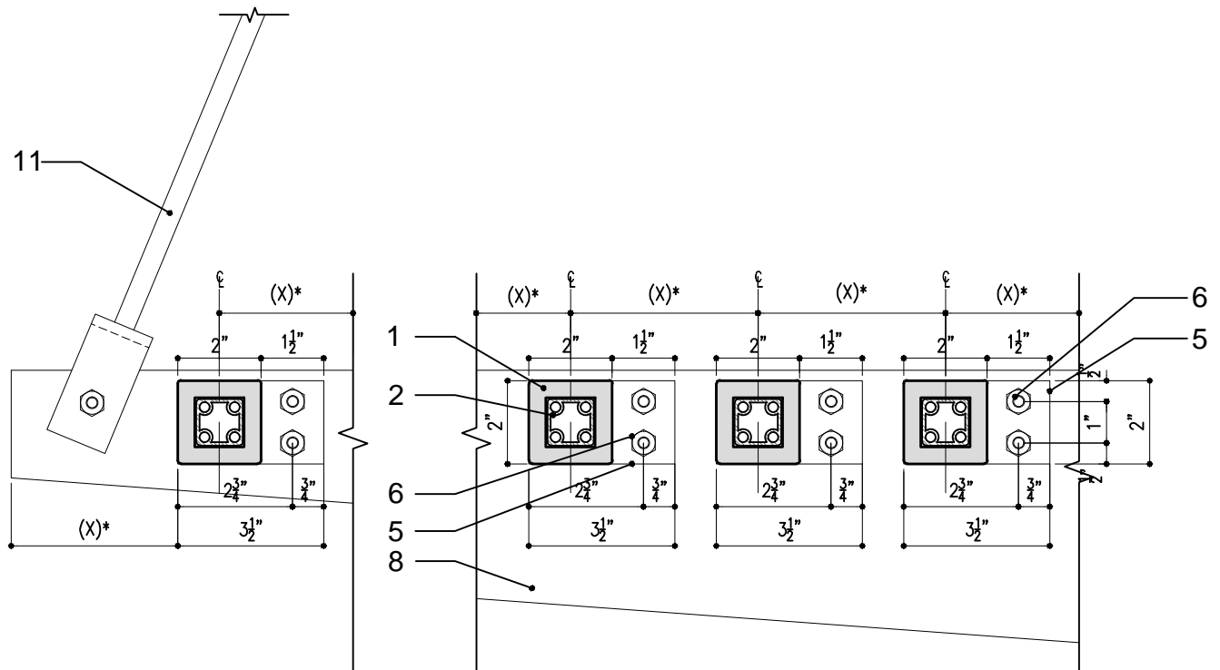
① SECTION DETAIL-THROUGH TILE
