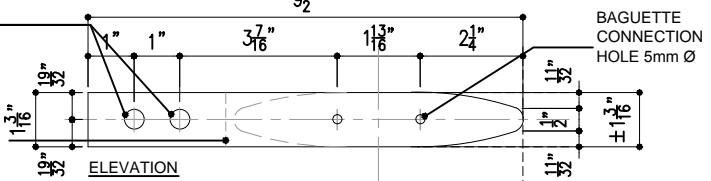
2D END PLATE 2 (OPTIONAL) CUSTOM LASER CUT
