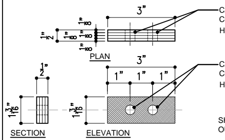
2C SHIM 2 (OPTIONAL)
