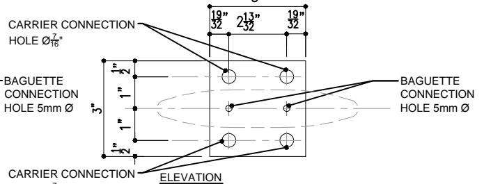
1D END PLATE 1
