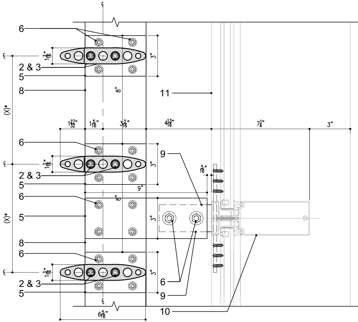
① SECTION DETAIL - LAMELLE TILE
