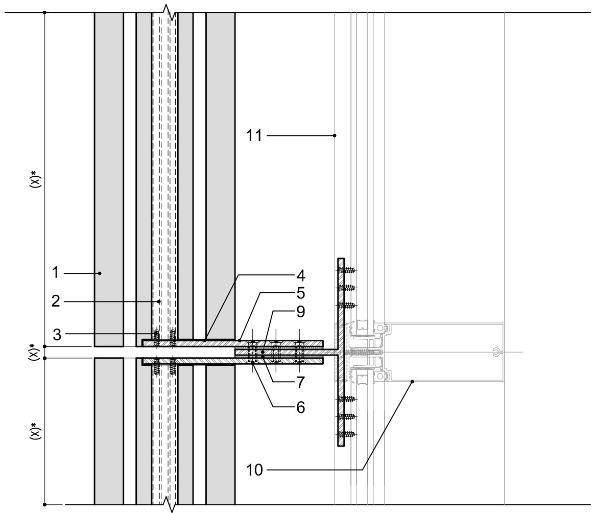
① SECTION DETAIL - LAMELLE TILE
