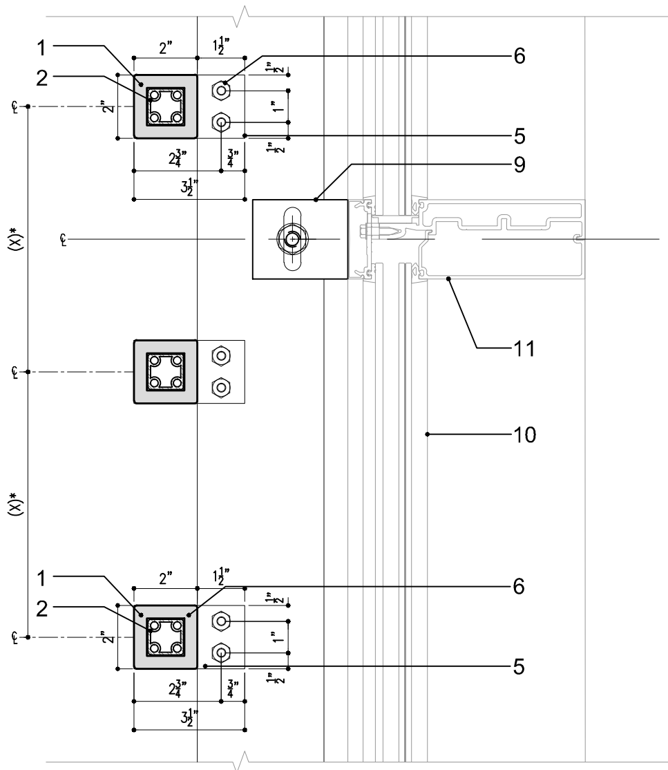
1 SECTION DETAIL - AT CURTAIN WALL
