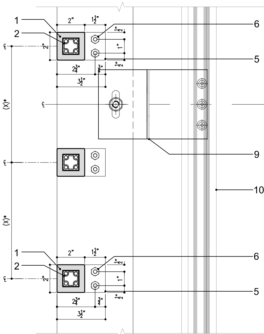
1 SECTION DETAIL - AT CURTAIN WALL
