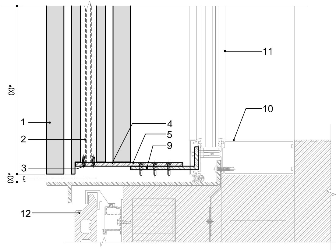
① SECTION DETAIL - SILL DETAIL
