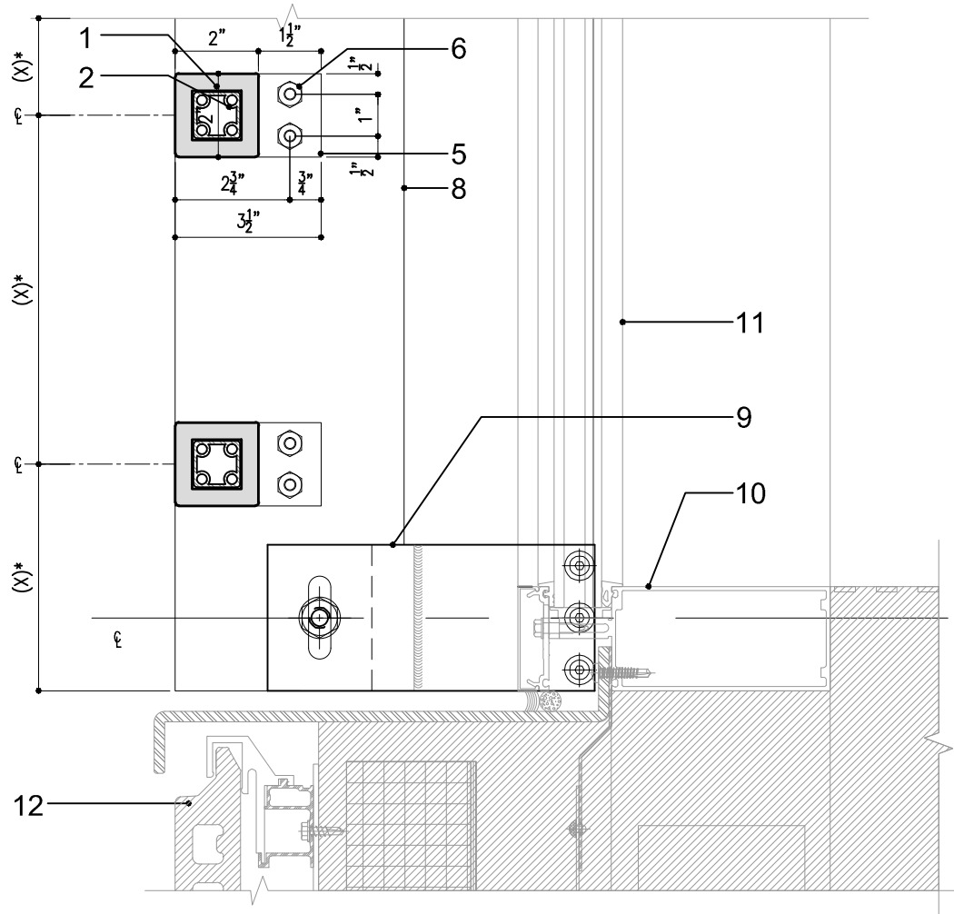
① SECTION DETAIL - SILL DETAIL
