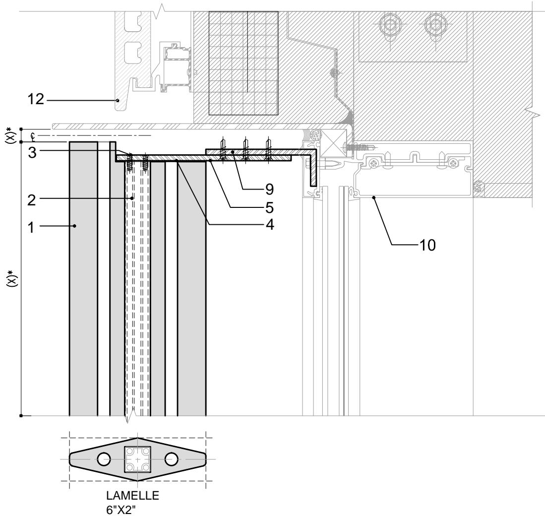
① SECTION DETAIL - HEAD DETAIL
