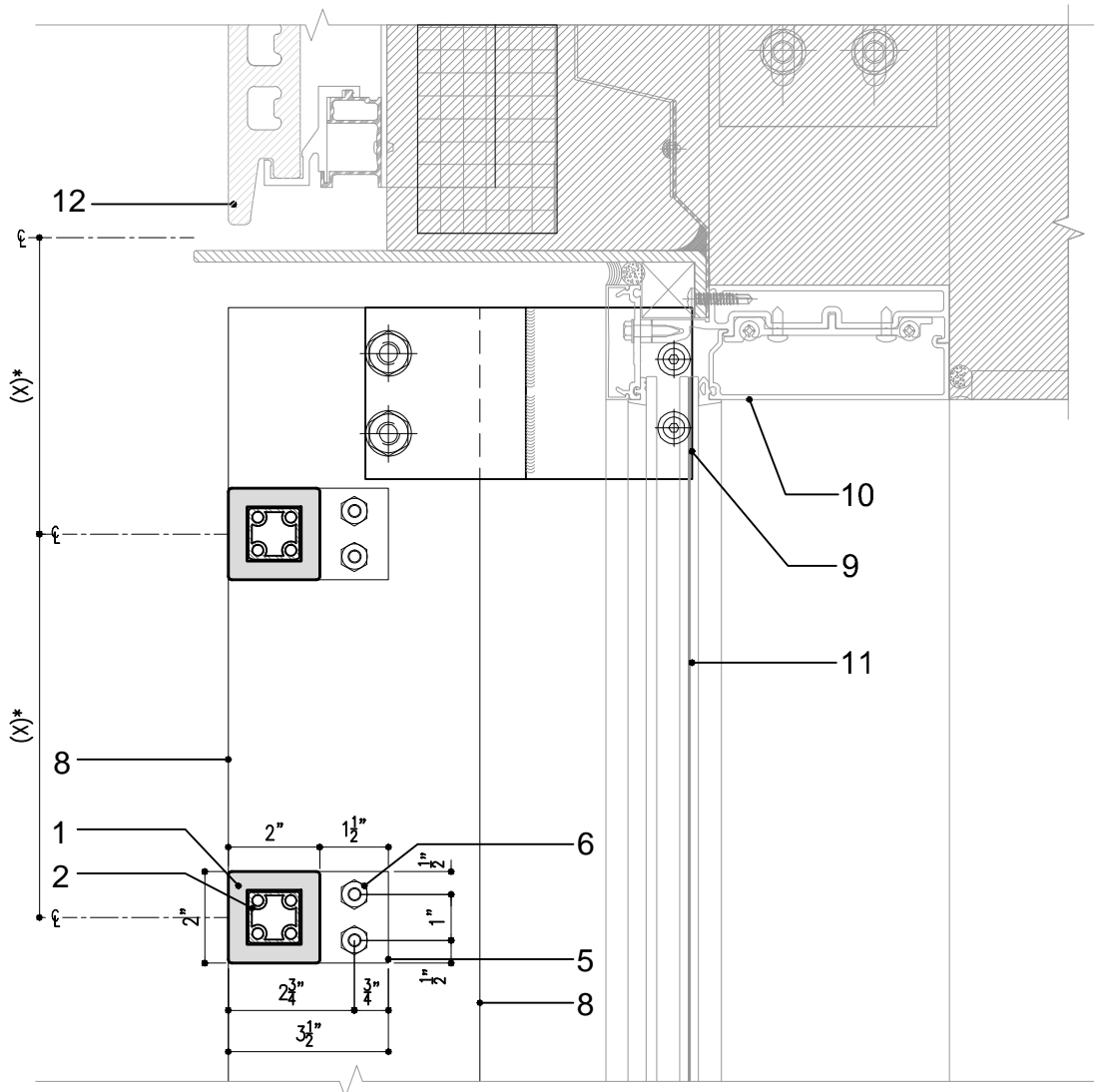
1 SECTION DETAIL - HEAD DETAIL
