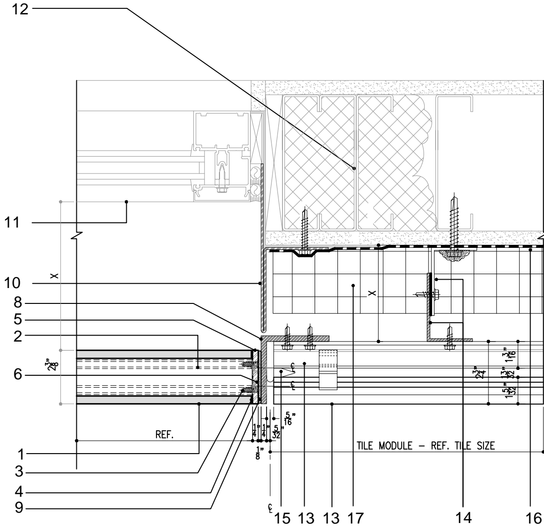
1 PLAN DETAIL - AT BAGETTE
