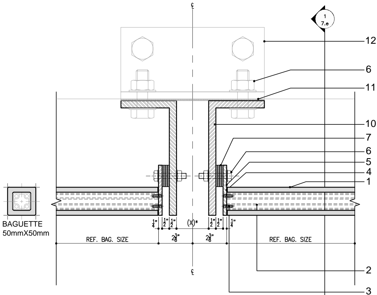
1 PLAN DETAIL - AT FREE STANDING STRUCTURE
