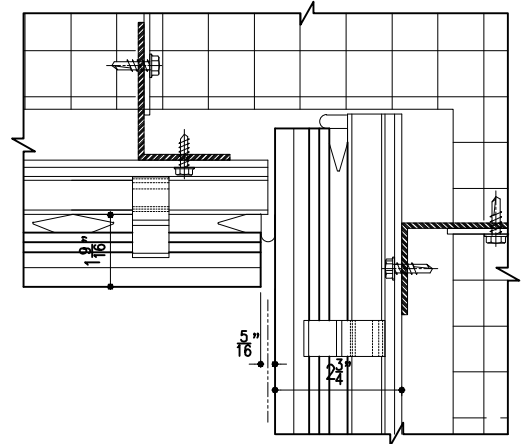
CORNER W/O TRIM CHANNEL
